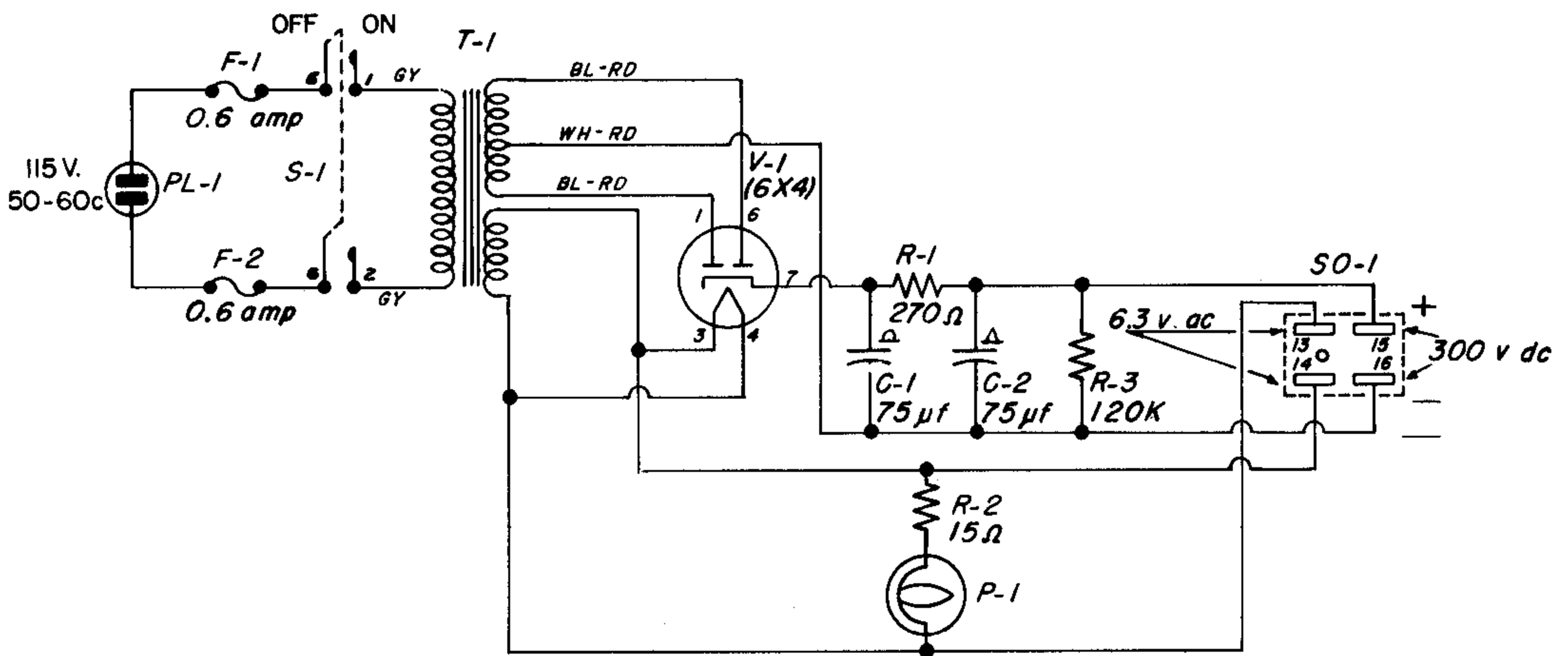
Figure 2. Schematic Diagram.
